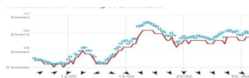
Wind 5 sep 2018
