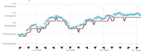
Wind 5 sep 2018
